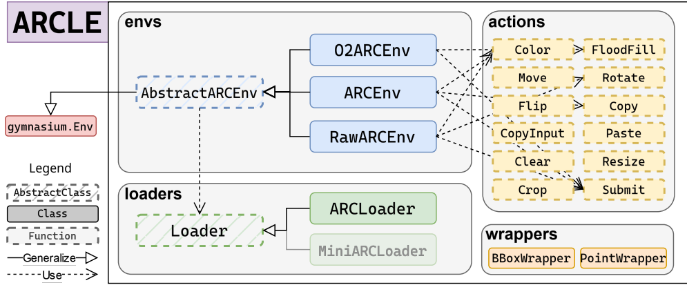
Figure 2: Framework of ARCLE. The package consists of envs, actions, loaders, and wrappers components.
